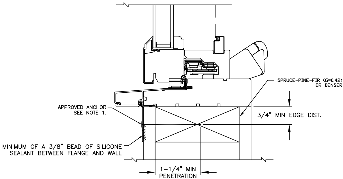
TYPICAL FLANGED WINDOW SILL
