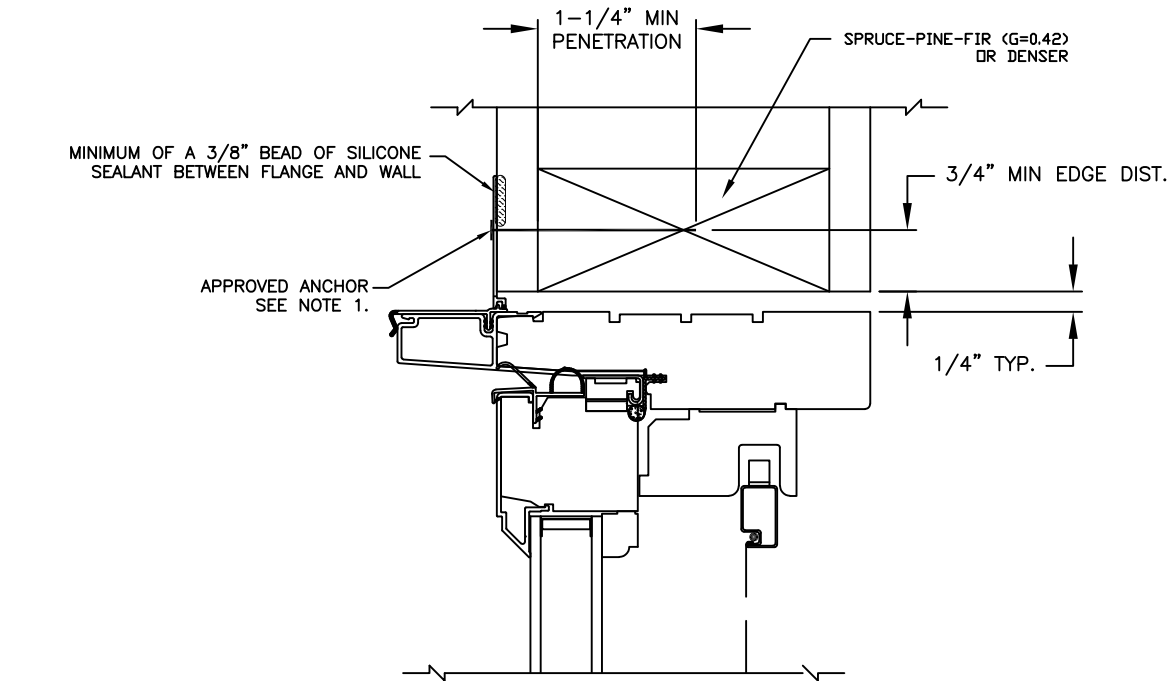
TYPICAL FLANGED WINDOW HEAD JAMB
